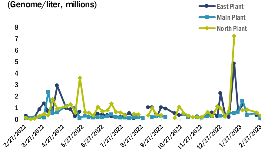
Burlington Wastewater SARS-CoV-2 Counts (Genome/liter, millions)
