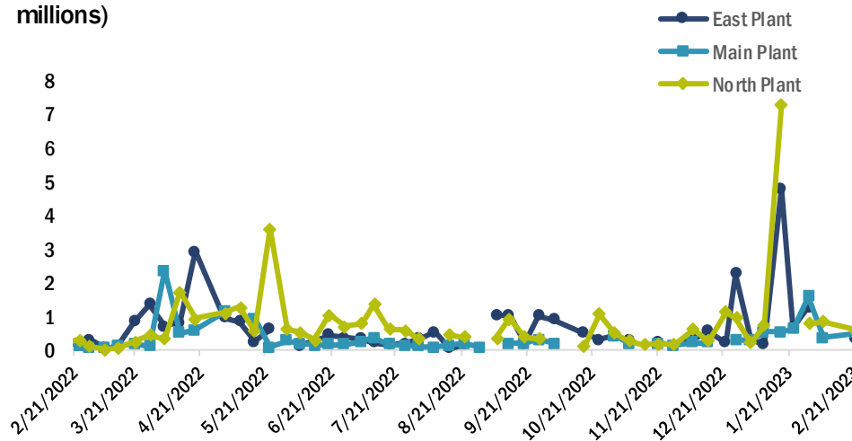
Burlington Wastewater SARS-CoV-2 Counts (Genome/liter, millions)
