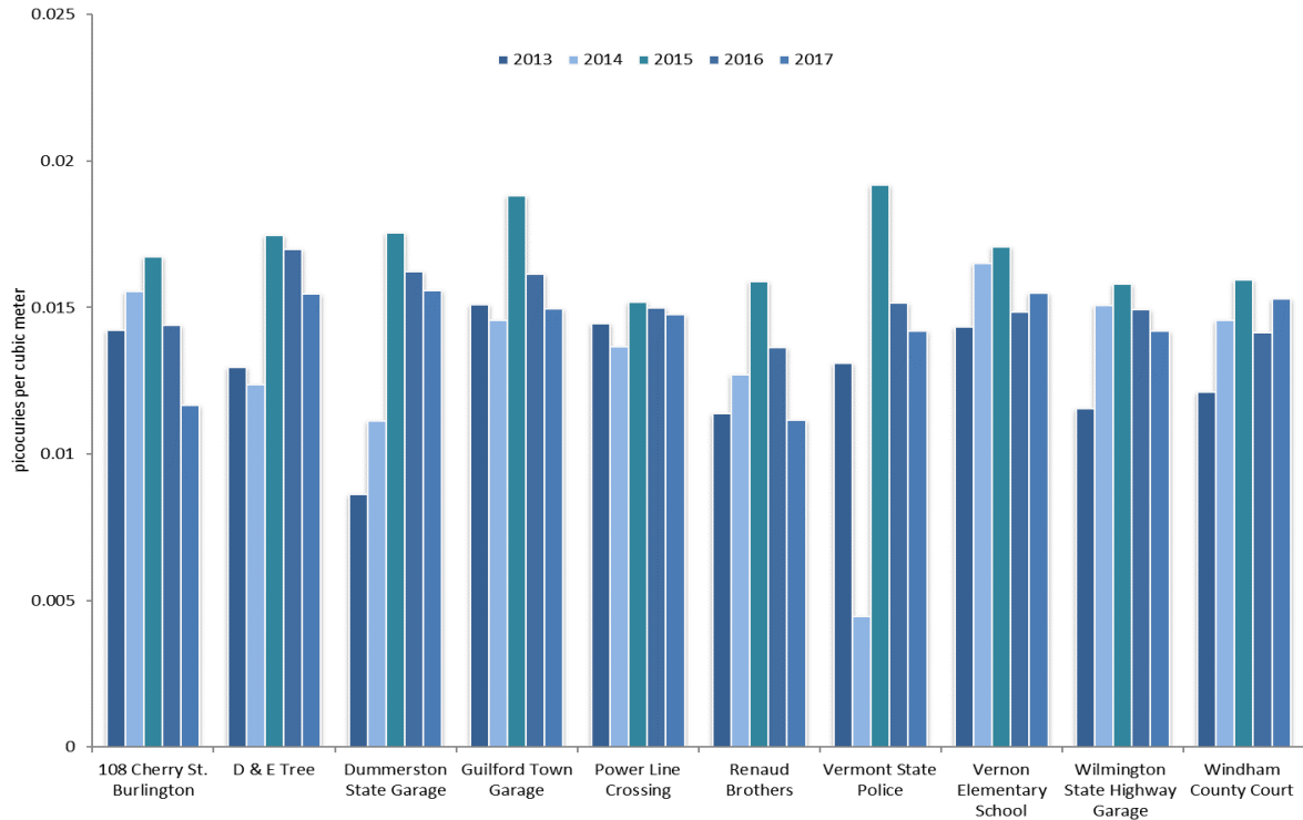
Figure 3. 2013-2017 Average Beta Radioactivity in Air
