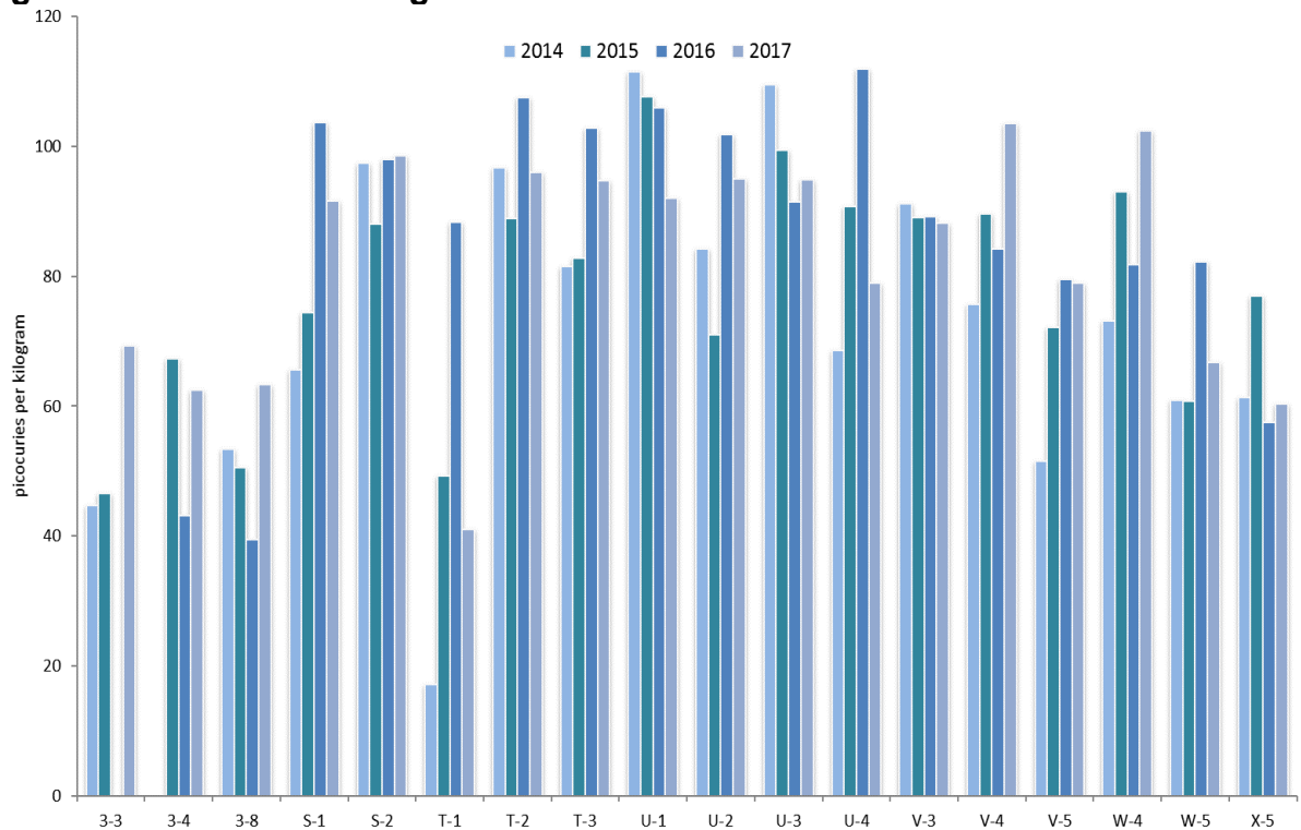
Figure 7. 2014-2017 Average Cesium-137 Levels in Sediment
